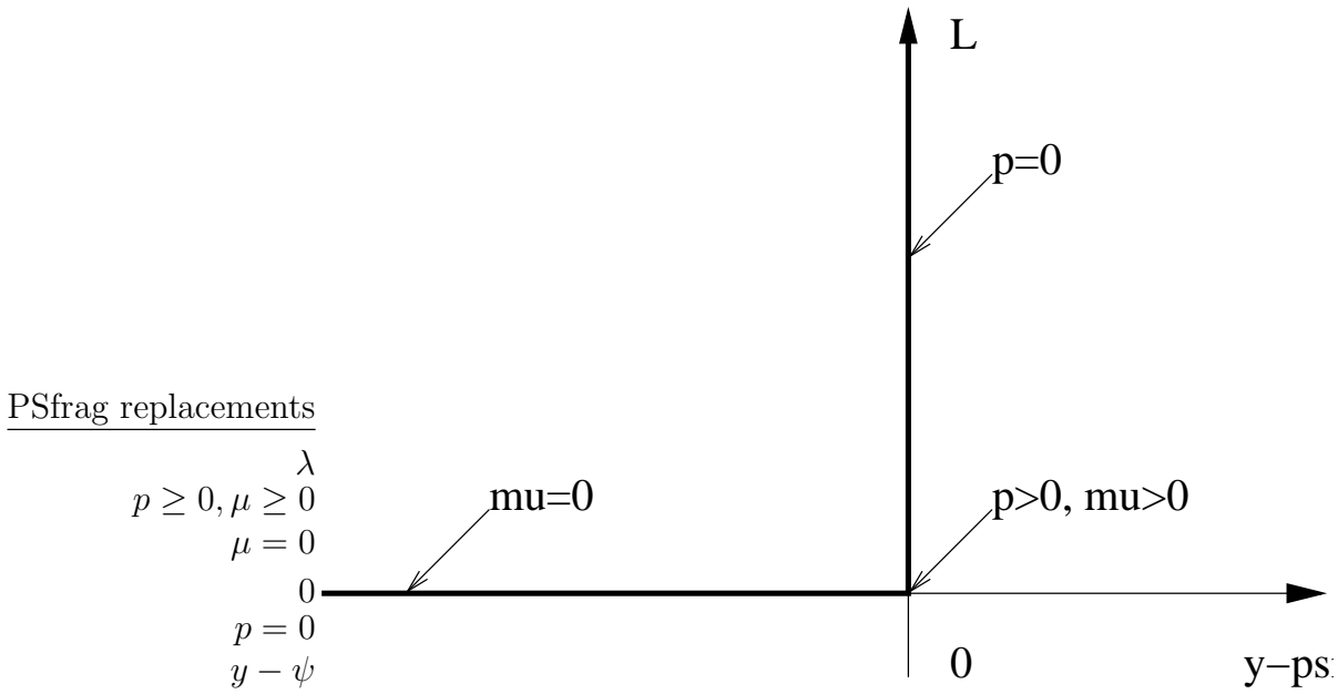
Figure 1: Complementarity relations
